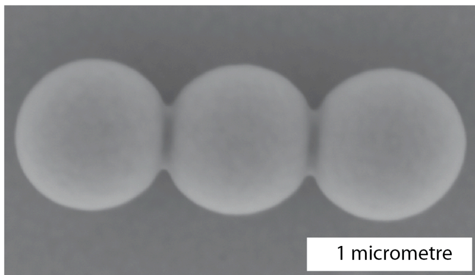
Figure 1 Field emission electron microscope image of water bridges connecting three silica spheres.
