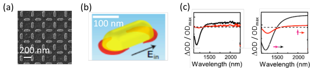
Figure1: (a) Example of a fabricated NA-VO 2 hybrid. (b) Simulated 68°C isosurfaces showing the phase-switched hot-spots around the nanoantennas generated by resonant pumping. (c) Difference in the OD of the antennas, induced by the hot-spots of (b), for both (black curves) parallel and (red curves) perpendicular pump-probe polarization. (left) Experiments and (right) simulations.
