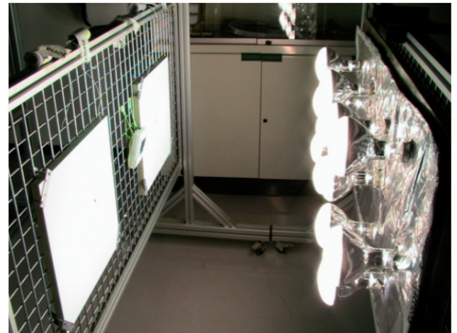
Figure 10: Solar simulator
