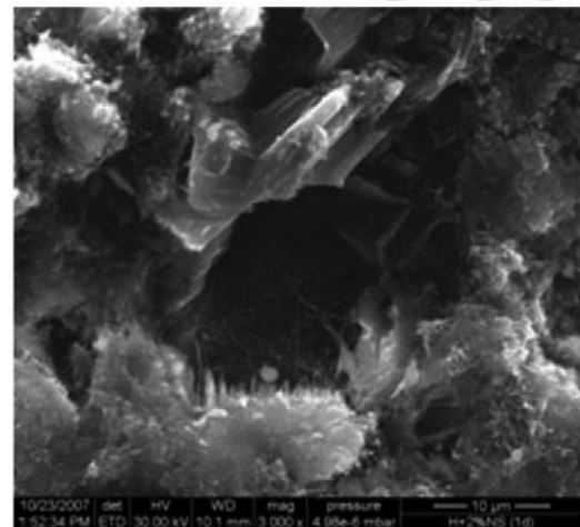
Figure 14: Cement hydration products and sepiolite
