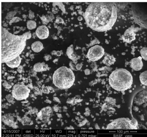
Figure 13: SEM image. Microencapsulate
