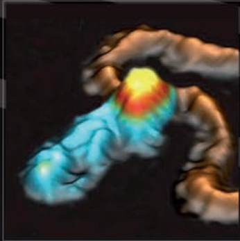
Single human Rad50/Mre11 protein complex bound to a DNA molecule. Image size 100 nm x 100 nm Moreno-Herrero et al. Nature. 437, 440-443 (2005).
