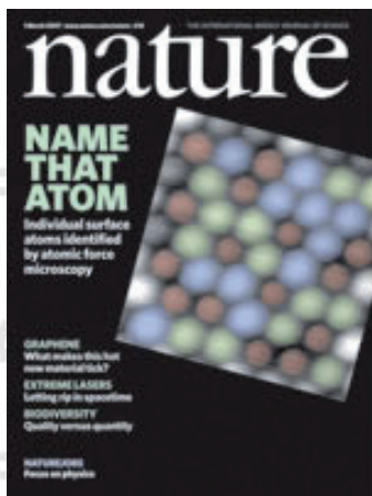
Copyright Macmillan Publishers Ltd 2007. Cover of the 2007, 1st of March issue of Nature devoted to the chemical identification of individual atoms by atomic force microscopy.
