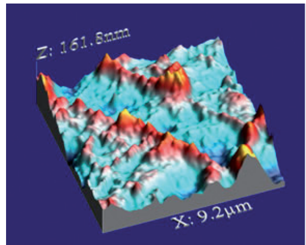
Atomic Force Microscope image of Polyamide with nanoparticles (Image size: 9,2 µm x 9,2 µm). Measured in Dynamic Mode. Courtesy of GAIKER (Bilbao, Spain)
