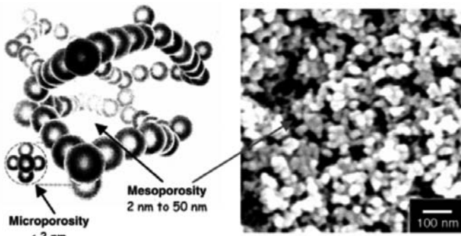
Figure 12: Aerogel structure.
