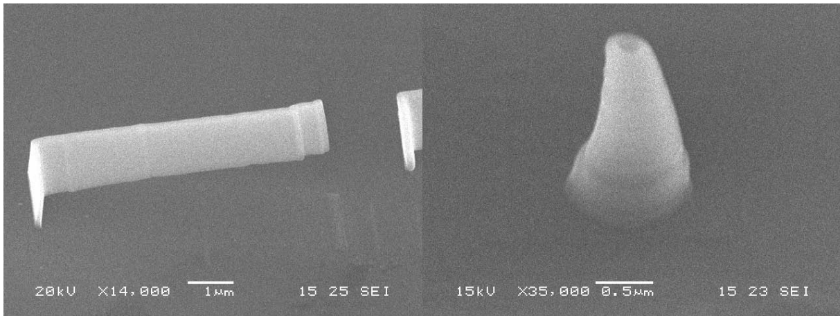
Fig N°1 Autosupported carbon membrane Fig N°2 Nanoinjector
