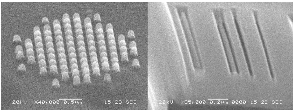
Fig N°3 Network of dots Fig N°4 Mask designed by FIB milling of a carbon membrane
