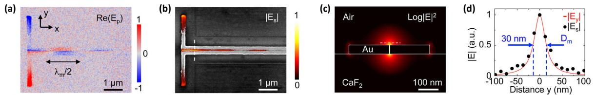
Fig. 1: Near-field imaging of a transmission line (TL) with a 5 nm gap. (a) Experimental near-field image showing the real part, \text{Re}(E_p) . (b) Experimental near-field amplitude image |E_s| superposed on the SEM image (grey color). (c) Numerically calculated mode profile. (d) Near-field amplitude |E_s| perpendicular to the TL extracted along the dashed lines in (b,c) (dots: experimental data, line: calculation), revealing an infrared mode diameter of only 30 nm. Imaging wavelength was \lambda_0 = 9.3 \mu\text{m} .
