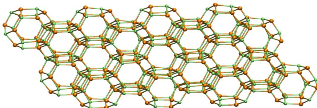
Figure 1: Characterized metastable FAU polymorph build by Cd_{12}S_{12} clusters.
