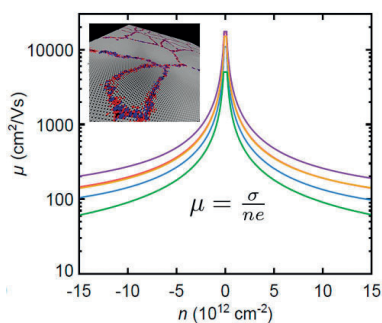
Simulated charge mobility of polycrystalline graphene. D.V. Tuan, J. Kotakoski, T. Louvet, F. Ortmann, J. C. Meyer, and S. Roche, Nano Letters , 13(4), 1730-1735 (2013)
