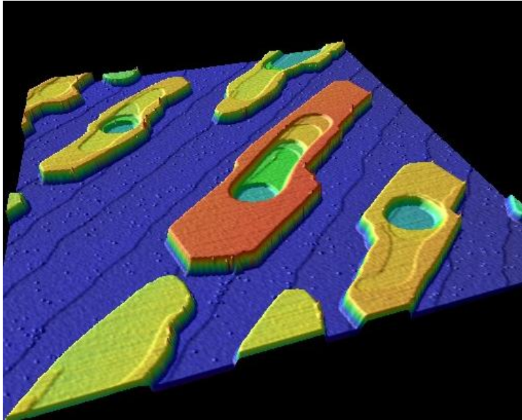
Figure 1. STM-image (600nm x 600nm) of the studied system. The network consists of mono-atomic terraces of Si-substrate covered by non-superconducting wetting layer of Pb (in blue) and superconducting Pb-nano-islands few monolayer thick (green-yellow-orange). Rich island geometry provides a variety of landscapes confining quantum vortices.
