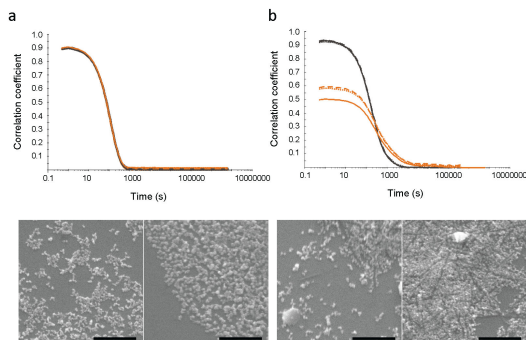
Fig. 3 > Behavior of TMV-SA- \mu MACS ® aggregates of 30 ng TMV / \mu l \mu MACS ® in an oscillating magnetic field ( H=1000 Oe, \nu=10000 Hz, U_{rel}=5 V). a: TMV Cyst (non-biotinylated, negative control); b: TMV Cyst-Bio (biotinylated). Upper panel: Correlograms (triplicates) of the dynamic light scattering of the aggregates before (grey) and after (orange) exposure to the oscillating magnetic field. Lower panel: ESEM images before (left) and after (right) exposure to the oscillating magnetic field. Bar = 500 nm./
