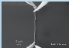
Direct 4-contact nanoprobng of an Au-capped Ni/NiO 2 nanowire
